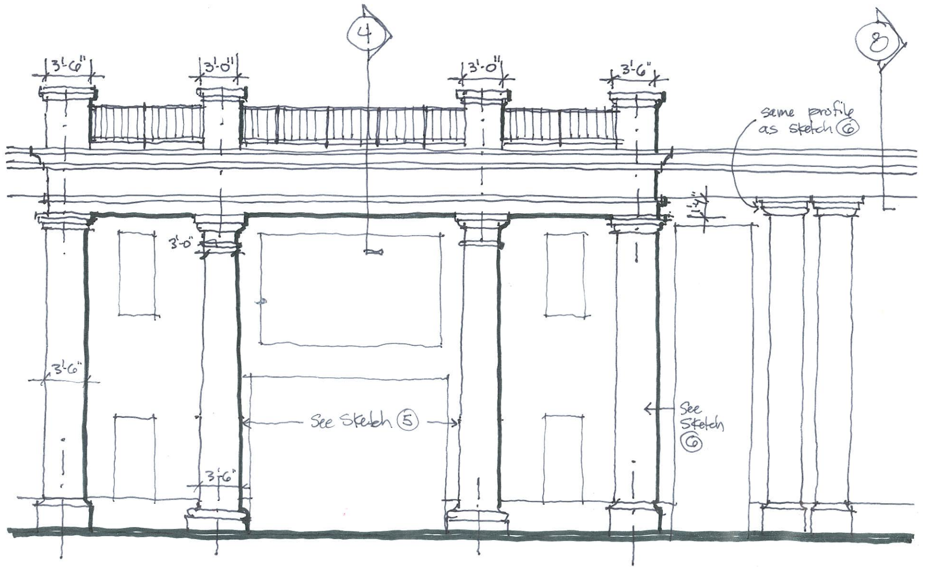
Elevation @ South Entry sc: 10" x 160"
